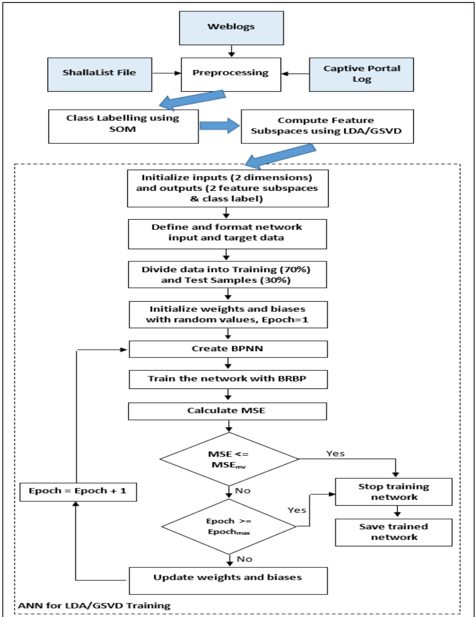
Figure 1. The training process for the development of the ANN for LDA/GSVD algorithm.
